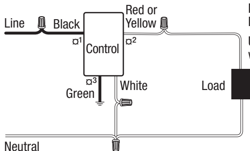
With Neutral
