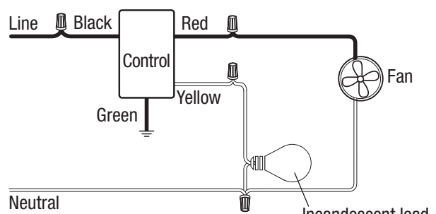
Fan/Light
