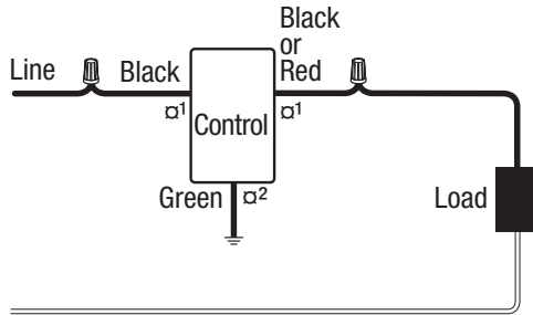
Single-Pole
