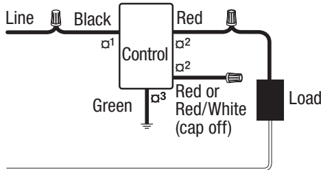
3-Way Control
